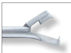
Tischler, Standard Down
